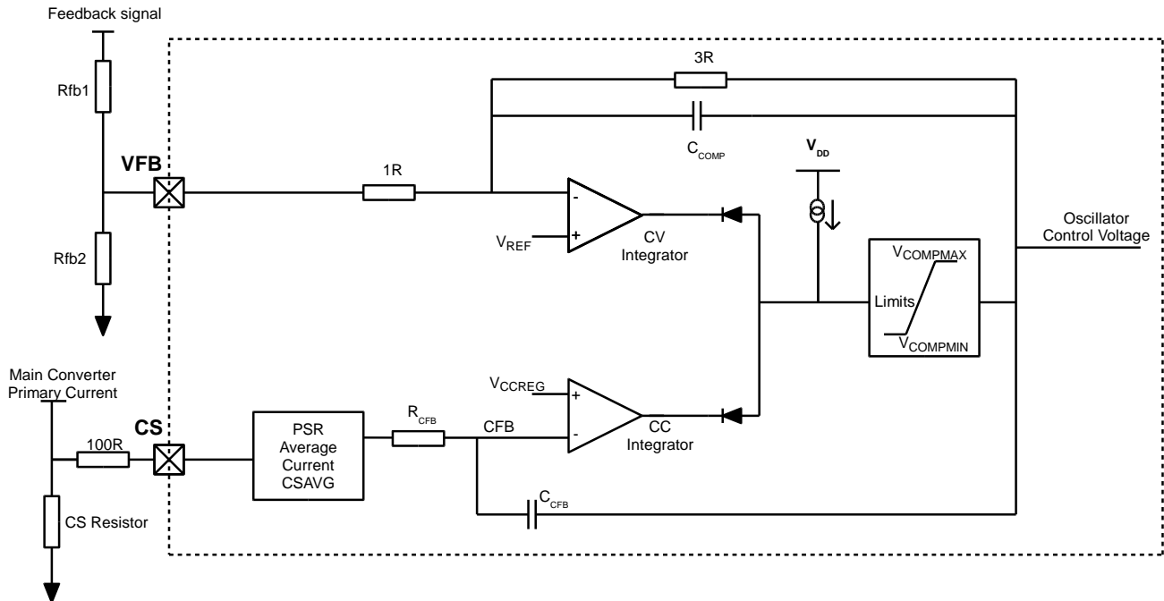
Figure 6: Error Amplifier Circuits
