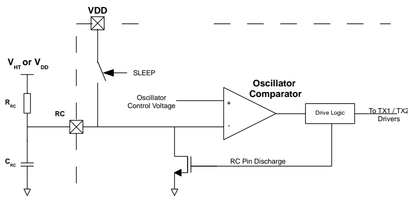
Figure 8: Oscillator circuit
