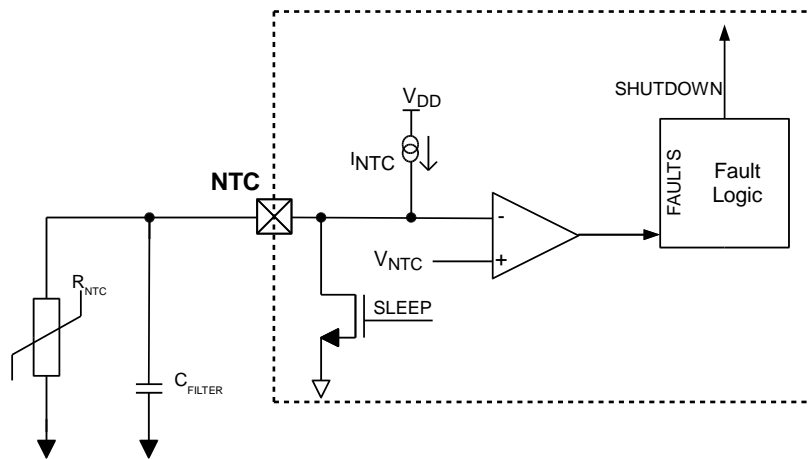
Figure 9: RED2541 NTC pin circuit
