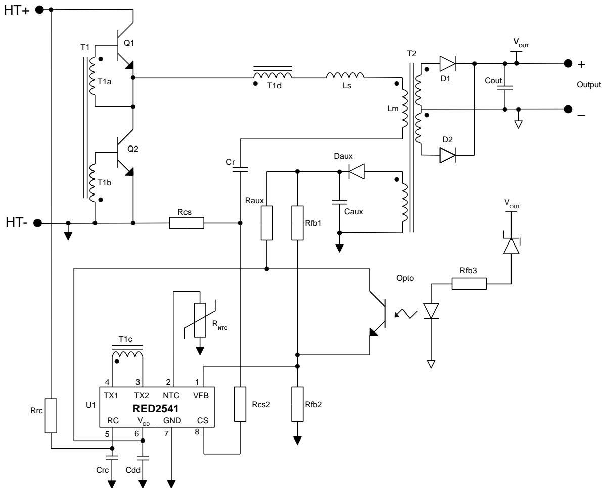
Figure 3: Typical Application Schematic: LLC converter with RED2541 CV controller
