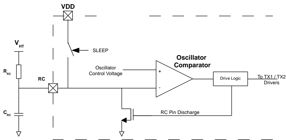
Figure 8: Oscillator circuit
