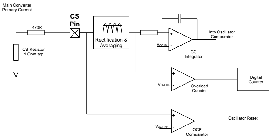
Figure 7: current protection circuits
