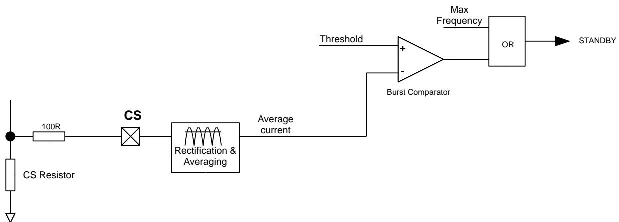
Figure 9: STANDBY entry circuit
