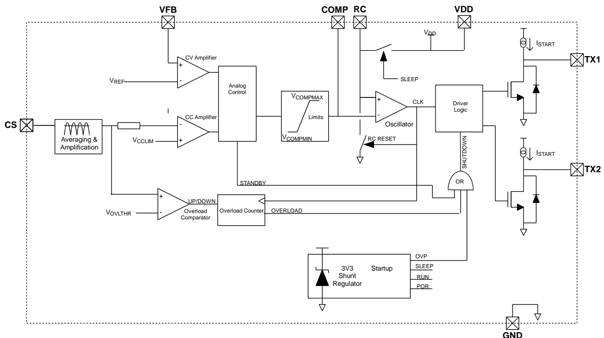
Figure 1: RED1501 Block diagram
