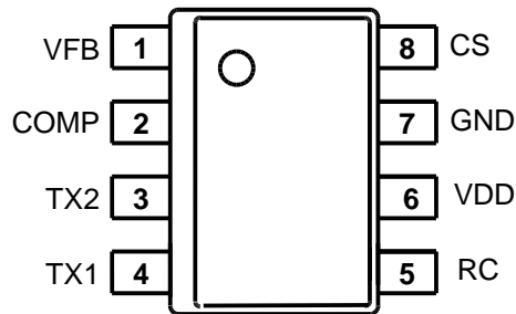
Figure 2: S08 pin connections (top view)
