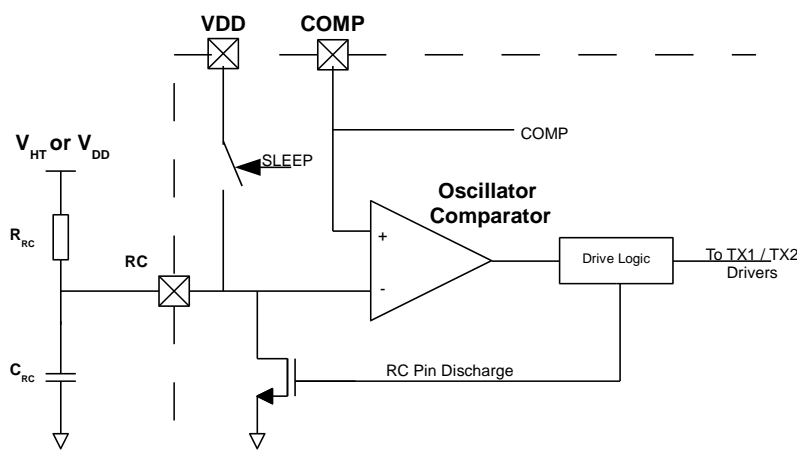
Figure 8: Oscillator circuit
