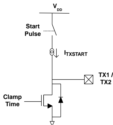
Figure 5: Drive Stage
