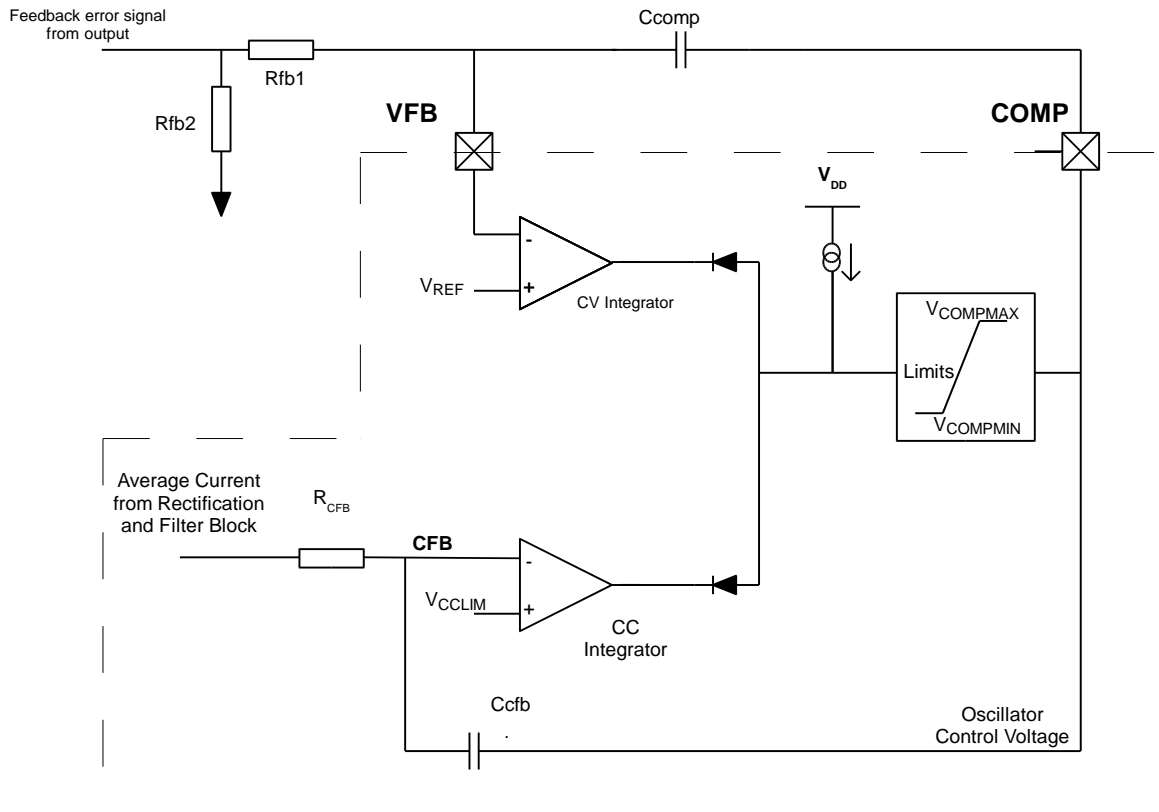
Figure 6: Error Amplifier Circuits
