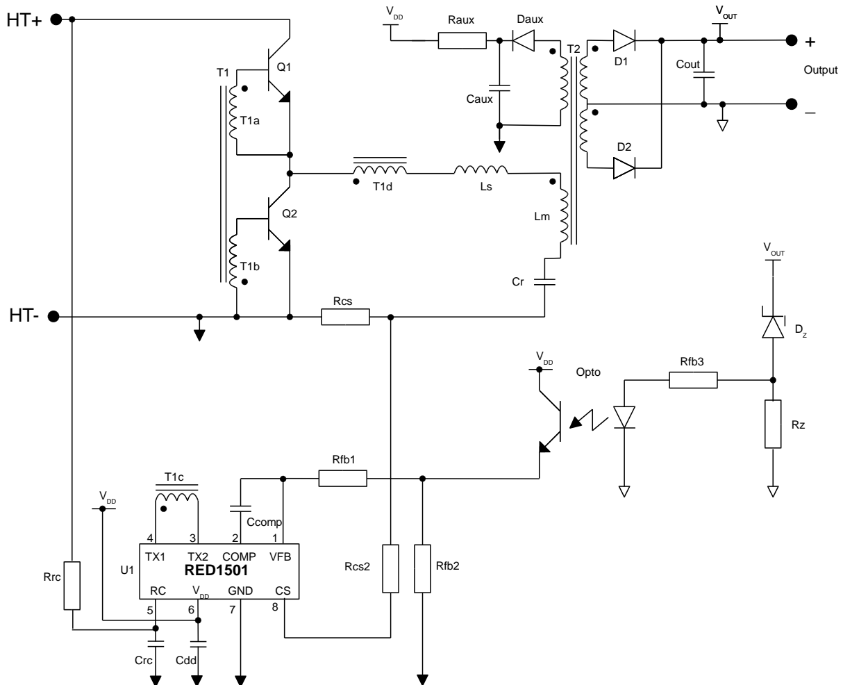
Figure 3: Typical Application Schematic using RED1501
