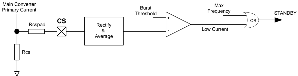
Figure 6: Standby Entry Circuit
