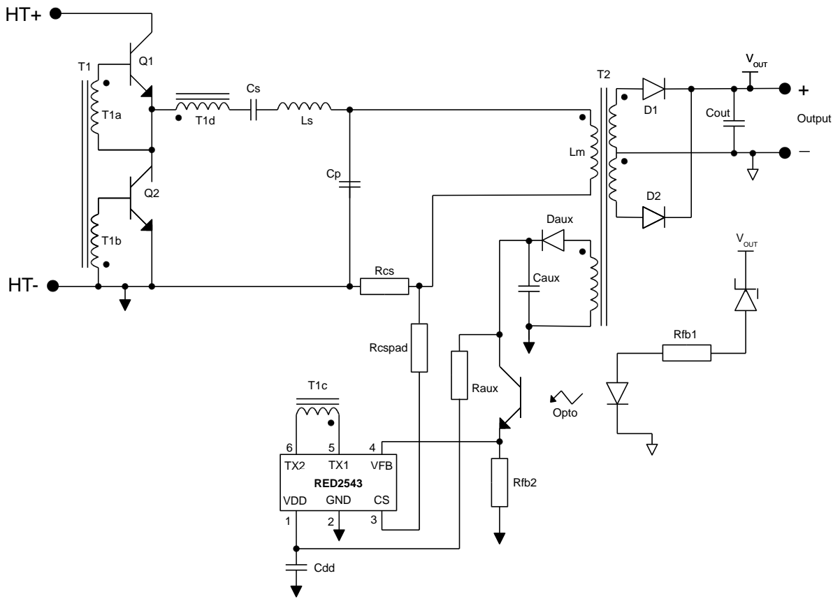
Figure 3: Typical Application Schematic: LLC converter with RED2543 CV controller
