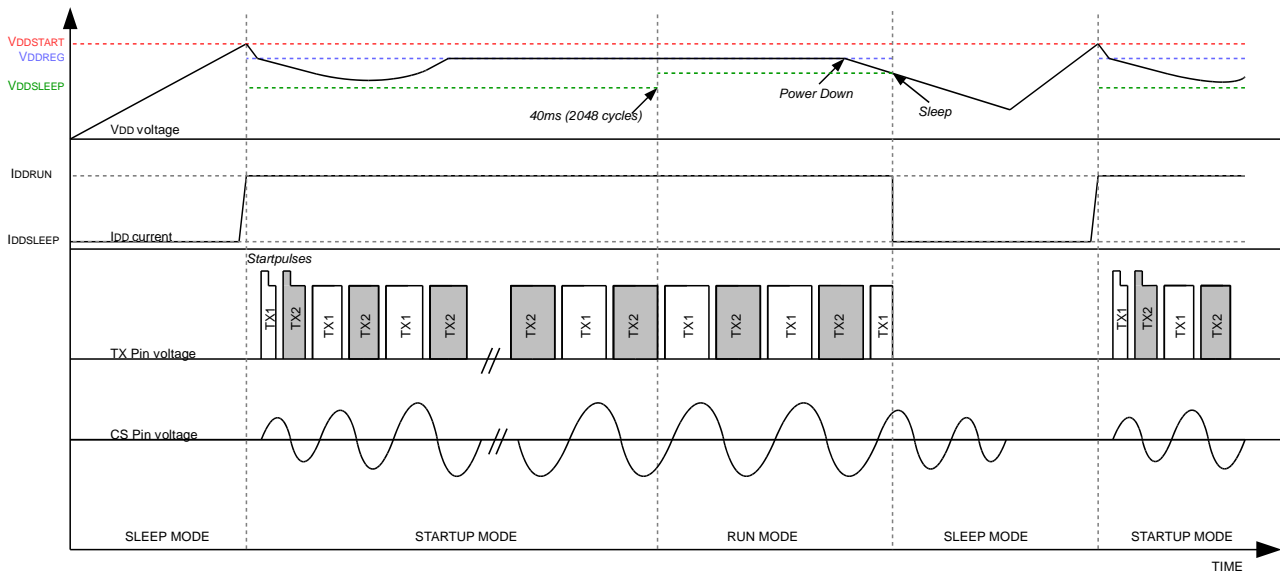
Figure 4: IC Start-up waveforms
